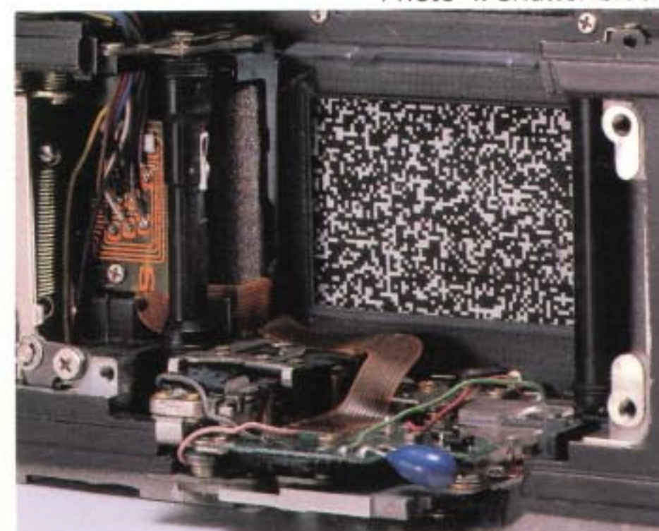
Photo 4. Shutter block
