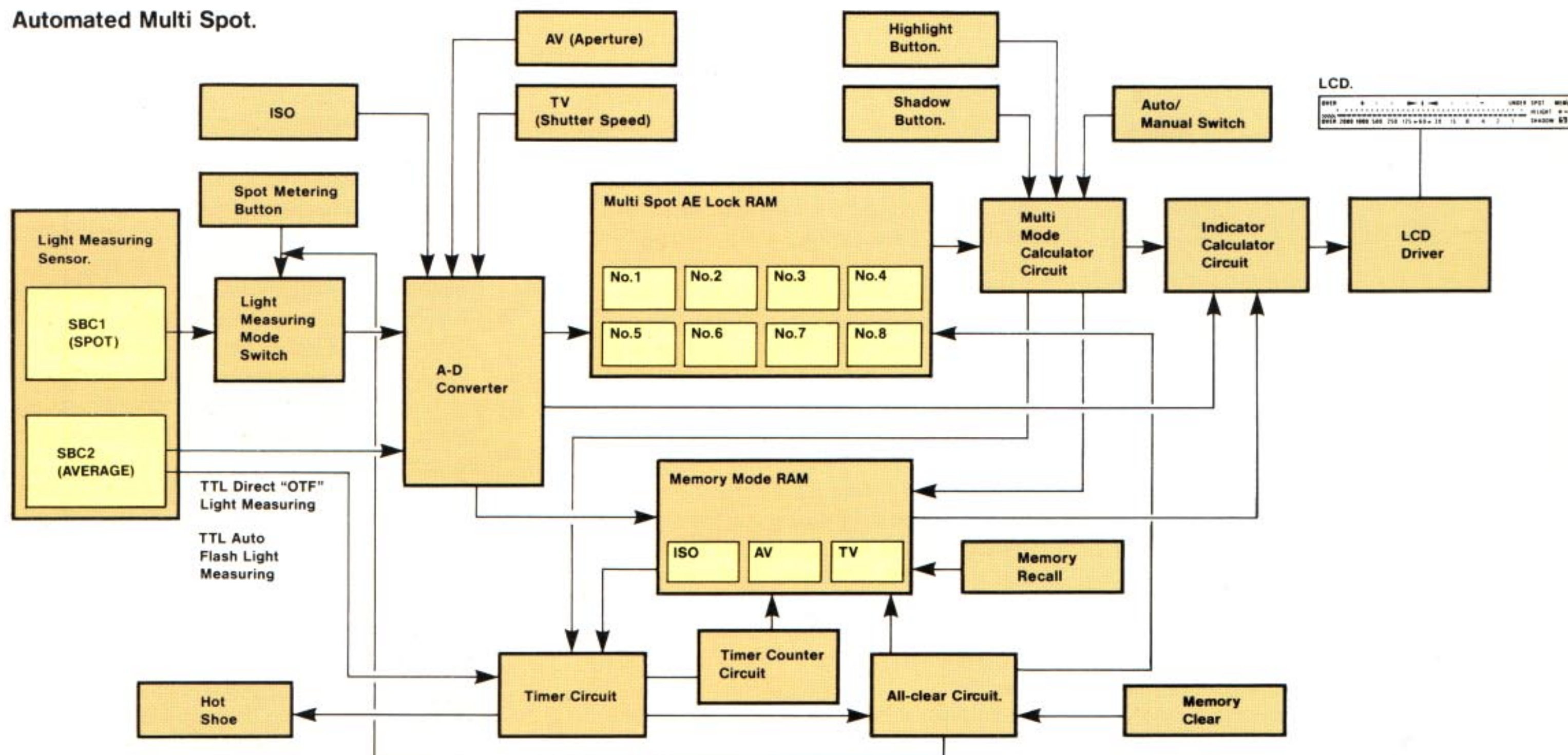
Diagram 7. Exposure control diagram
