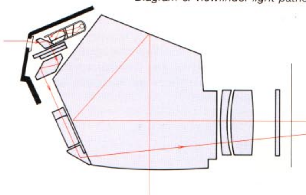
Diagram 6. Viewfinder light paths
