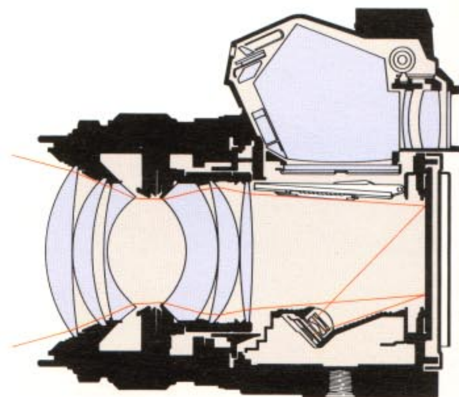
Diagram 2. TTL Direct "OTF" Light Measuring
