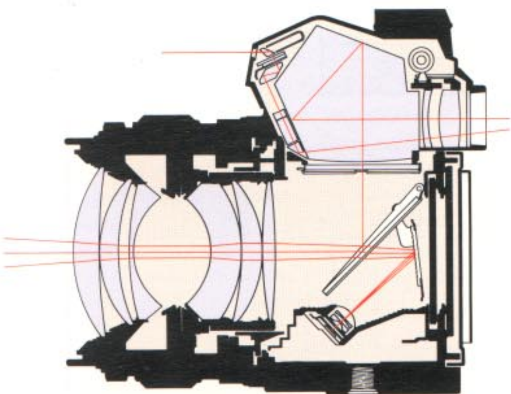
Diagram 4. Spot Metering
